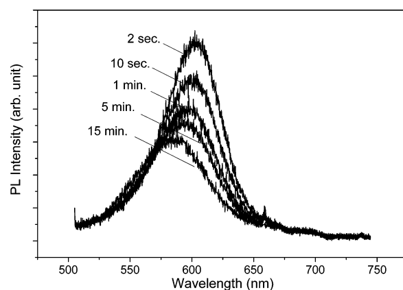
Figure 11. Time evolution of the PL spectra from the QDs in a \text{NaN}_3 -treated C2C12 cell.
