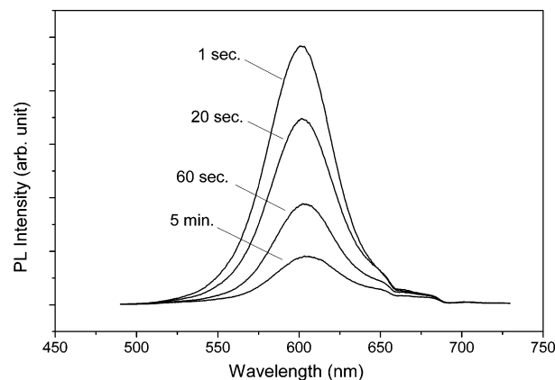
Figure 7. Time evolution of the PL spectra recorded from the QD aqueous solution with histidine added.
